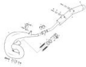
Escape
