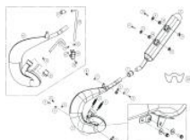
Escape
