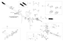
Manillar
