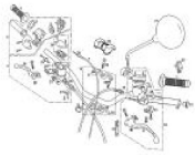
Manillar
